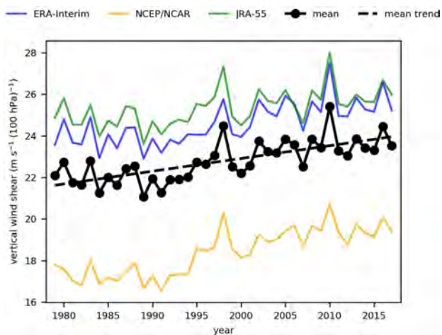
Extended Data Fig. 2 | Annual-mean regional-maximum six-hourly vertical shear in zonal wind in the North Atlantic at 250 hPa over the period 1979–2017. Data are presented from the ERA-Interim, NCEP/NCAR and JRA-55 reanalysis datasets. Also shown are the mean of the three reanalysis datasets and the linear trend in the mean.
