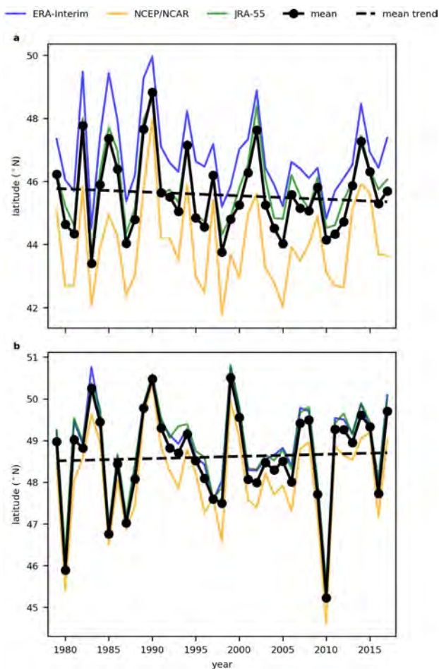
Extended Data Fig. 3 | Annual-mean latitude of the core of the polar jet stream in the North Atlantic at 250 hPa over the period 1979–2017.
