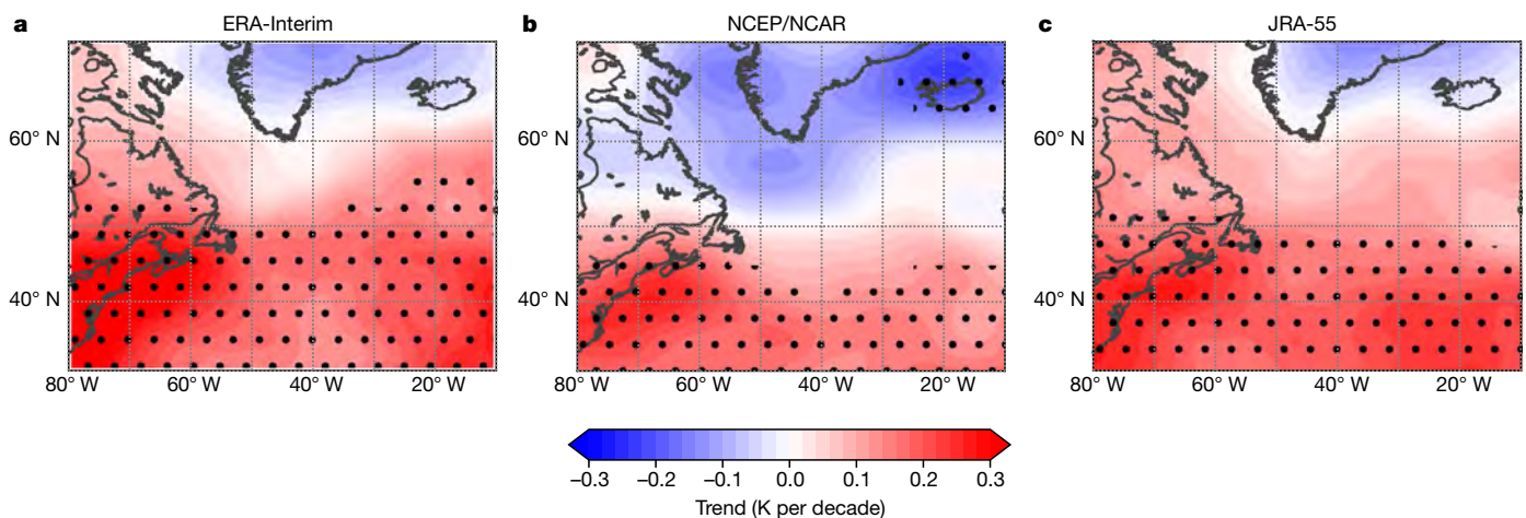
Fig. 1 | Annual-mean temperature trends in the North Atlantic at 250 hPa over the period 1979–2017. Linear trends are calculated using ordinary least-squares regression from the ERA-Interim (a), NCEP/NCAR
