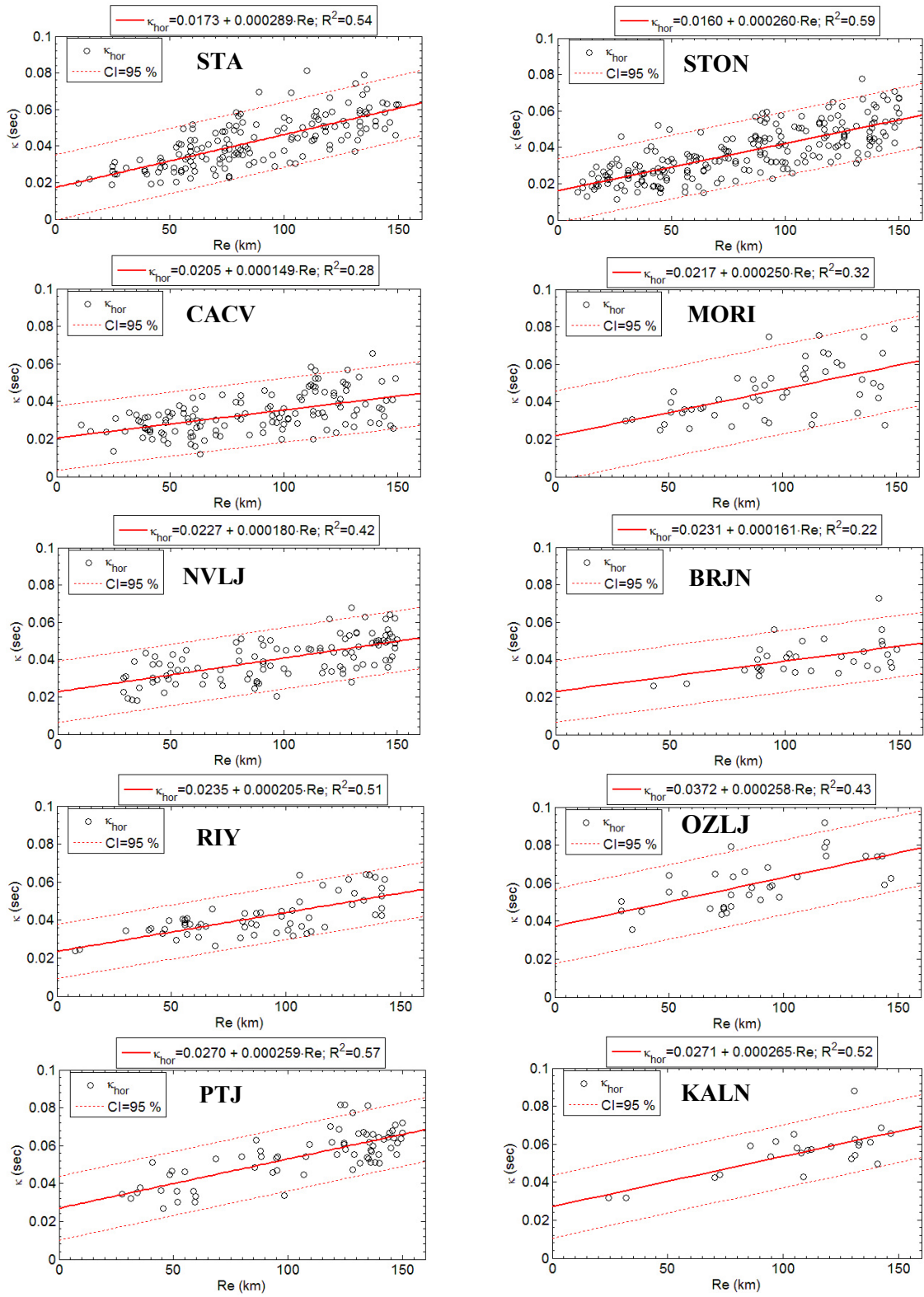
Figure 3. \kappa_{hor} model for Croatia as a function of a site (seismic station) and epicentral distance using standard linear regression (thick red line) with confidence interval (CI) of 95% (dashed line). Regression line equation (3) in term of \kappa_0 as zero R_E intercept and slope of regression in term of \kappa_R \cdot R_E with a coefficient of correlation R^2 is shown in legends.
