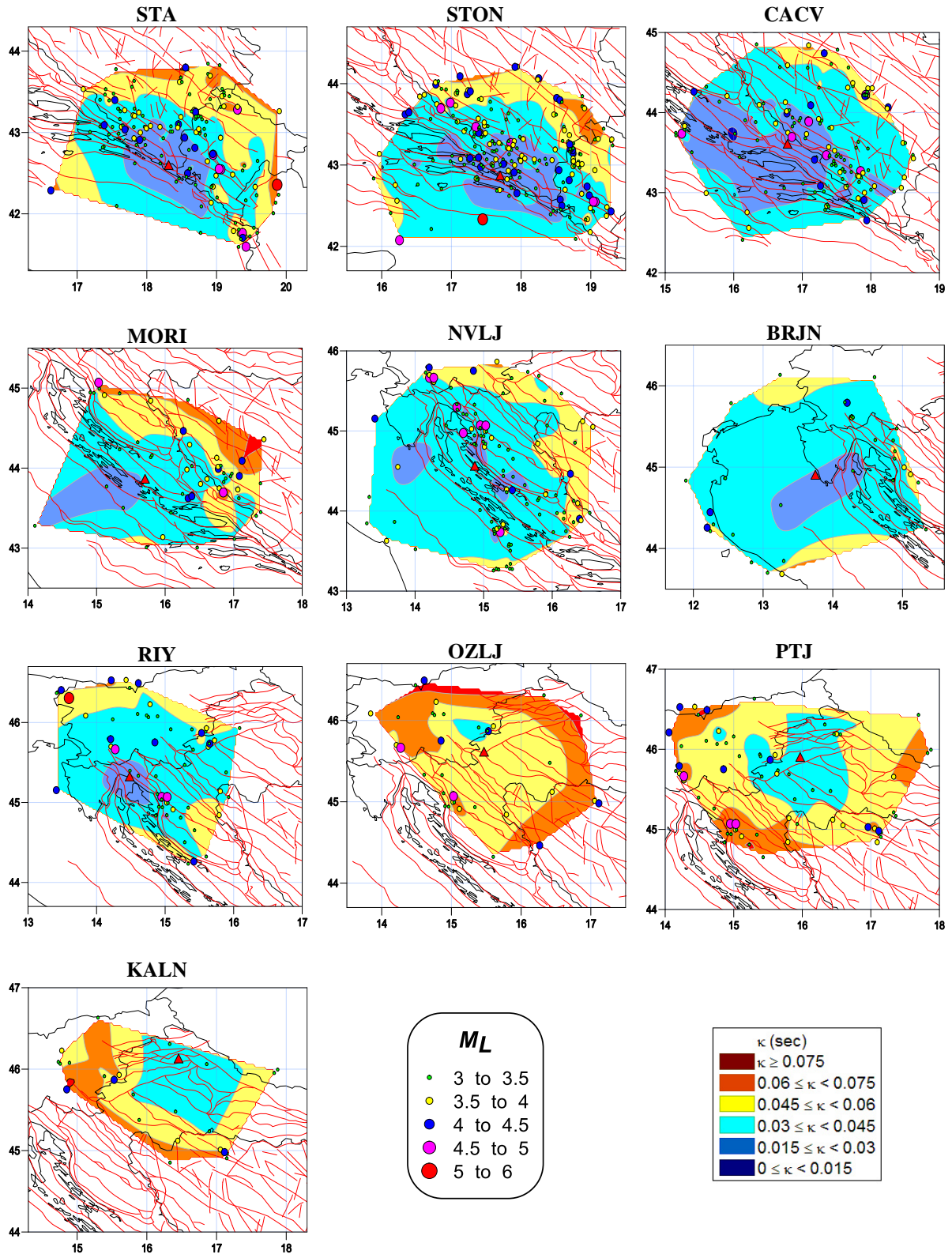
Figure 4. Spatial \kappa_{hor} distribution for seismic stations used in this research.
