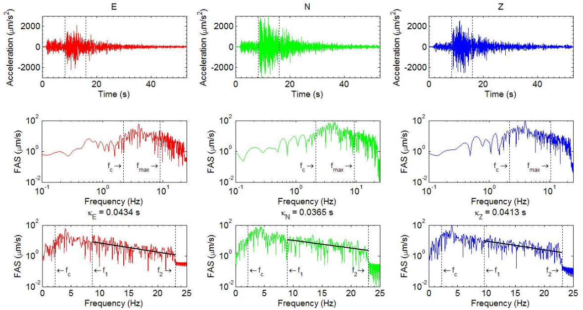
Figure 2: Example of kappa calculation using AH84 method for three component (E, N, and Z) seismogram. Station RIY, earthquake event on 16th June 2013 at 20:04, M_L=3.8 , R_E=56 km.
