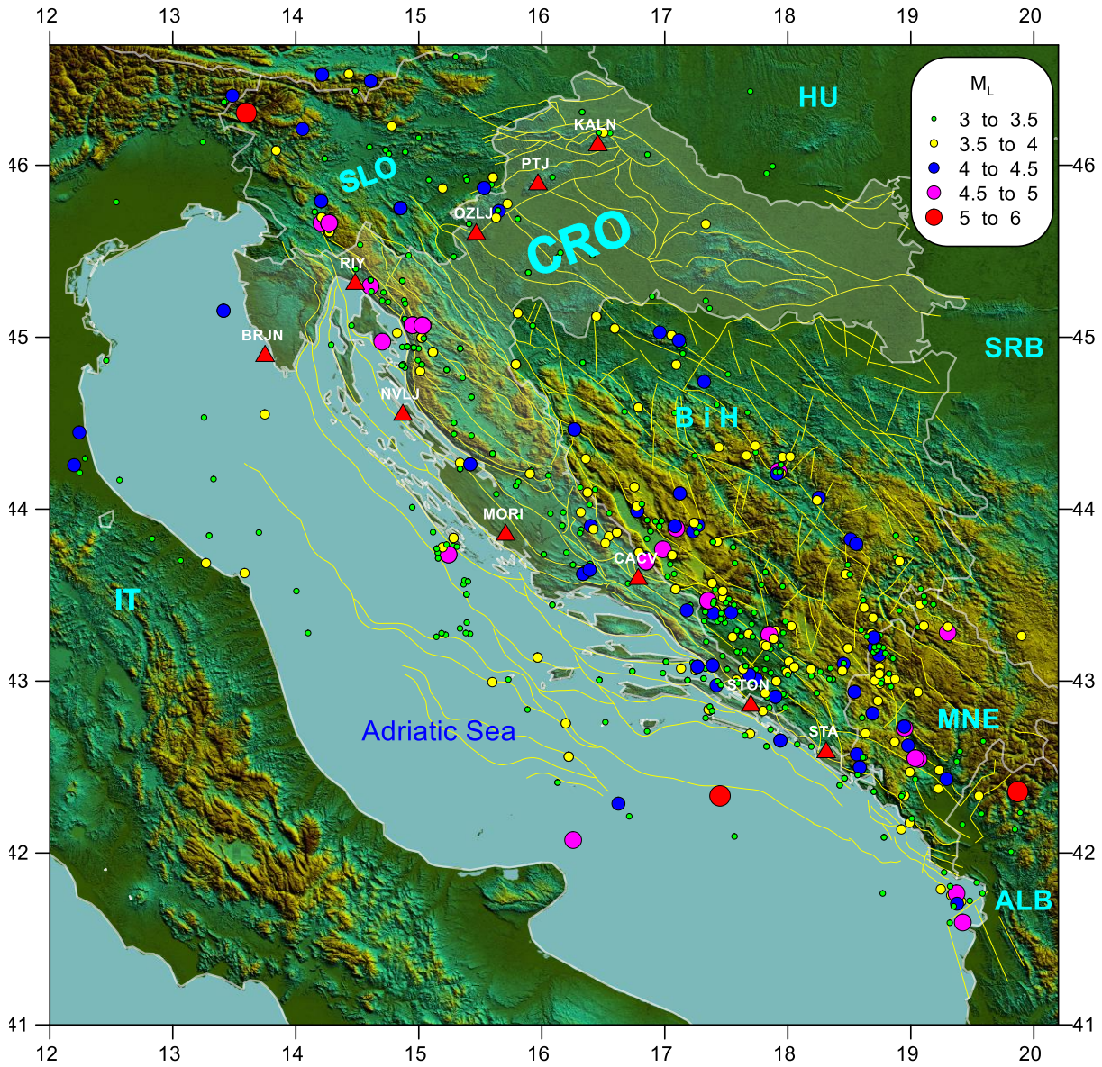
Figure 1. Map of earthquake epicenters (2002-2016) used in this study ( M_L \geq 3 , R_E \leq 150 km, and h < 30 km). Locations of seismic stations are marked with red triangles. Yellow lines represent known surface faults in Croatia and Bosnia and Herzegovina [6].
